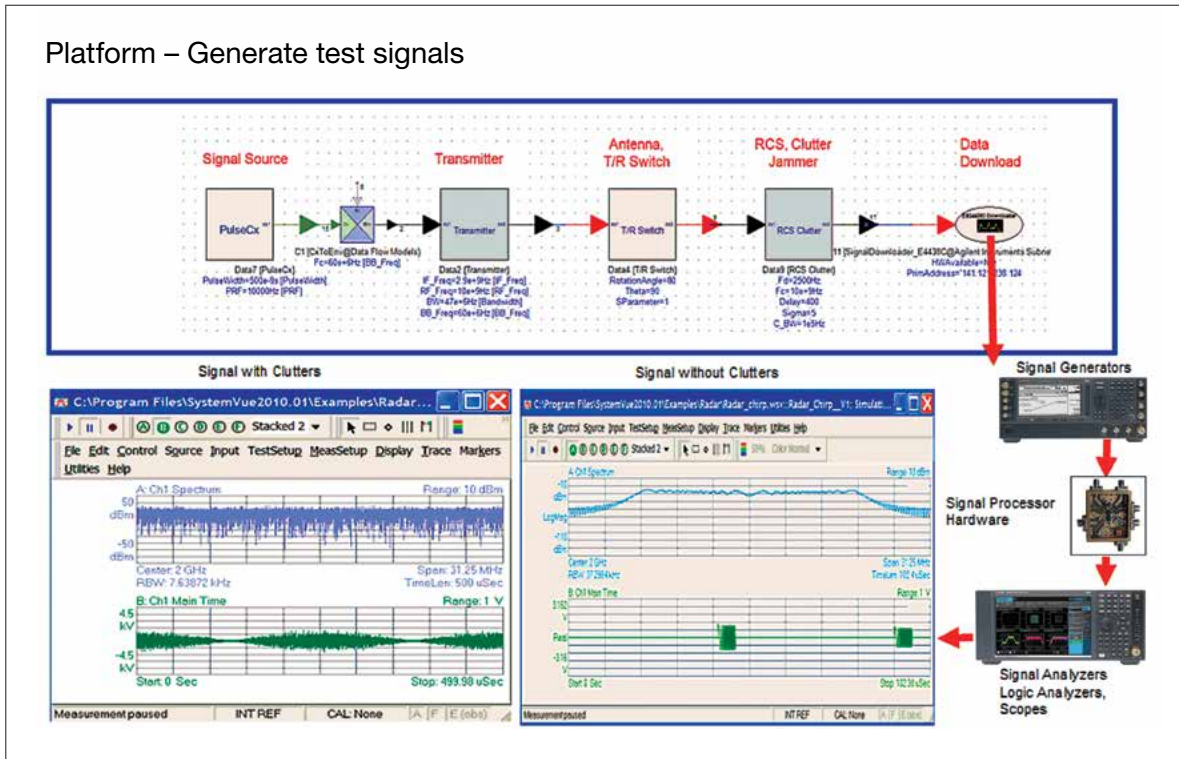
Figure 4.3. Generate test signals using SystemVue
