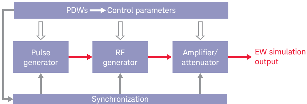
Figure 16.13. In the traditional approach, PDW control parameters are sent in parallel to multiple functional elements, on a pulse-to-pulse basis, to generate and modify the desired signal. This approach results in a complex system, demanding precise synchronization.
