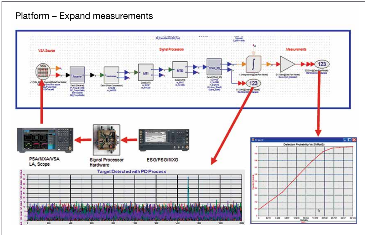
Figure 4.4. Expanding measurement capabilities using SystemVue
