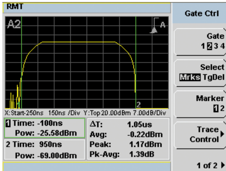
Figure 17.3. Using the P-Series peak power meter to measure peak power, gated pulse power, and peak-to-average ratio. Due to the shape of this pulse the peak power is 1.39 dB higher than the pulse power.
