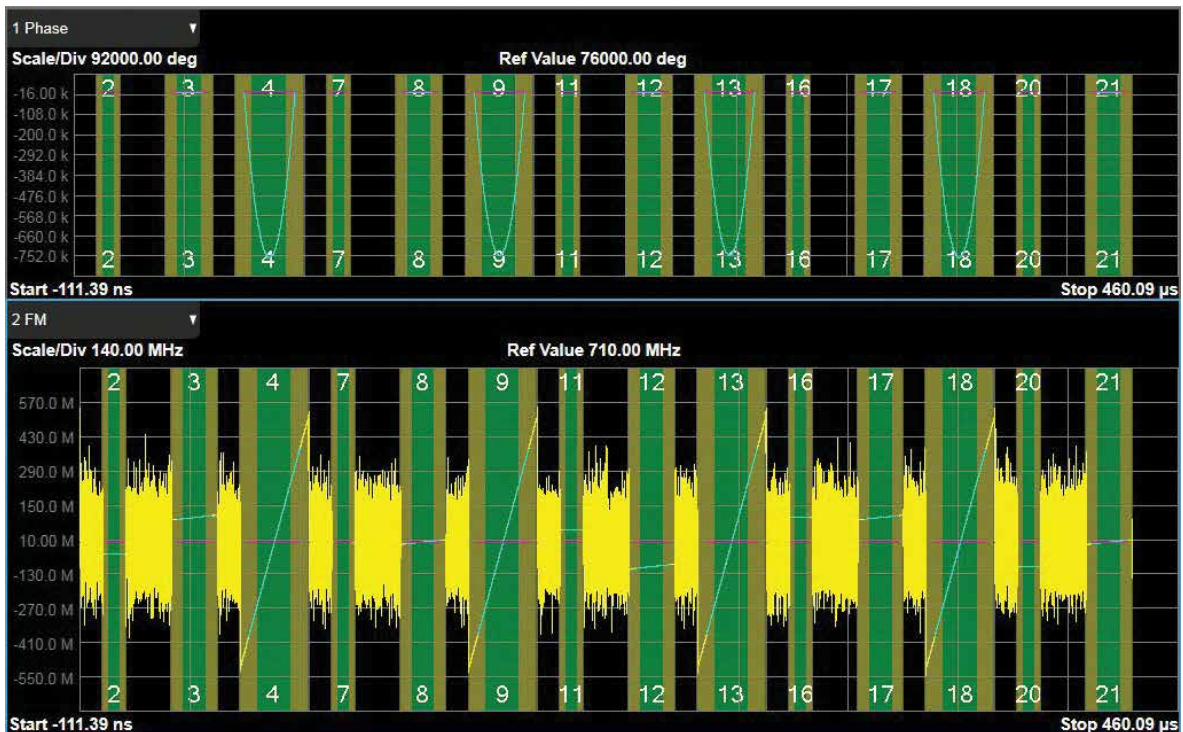
Figure 22.20. The UXA's wide integrated bandwidth simplifies the measurement of linear FM-modulated pulses.
