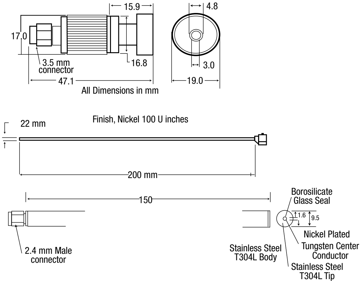
Figure 15.5. Coaxial probes
