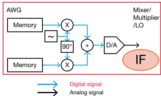
Digital baseband architecture
