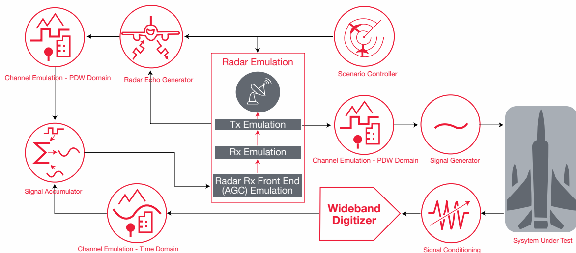
Figure 21.1. A candidate test system to evaluate jammer effectiveness
