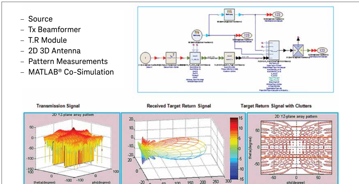
Figure 6.8. An example of array antenna pattern measurements.
