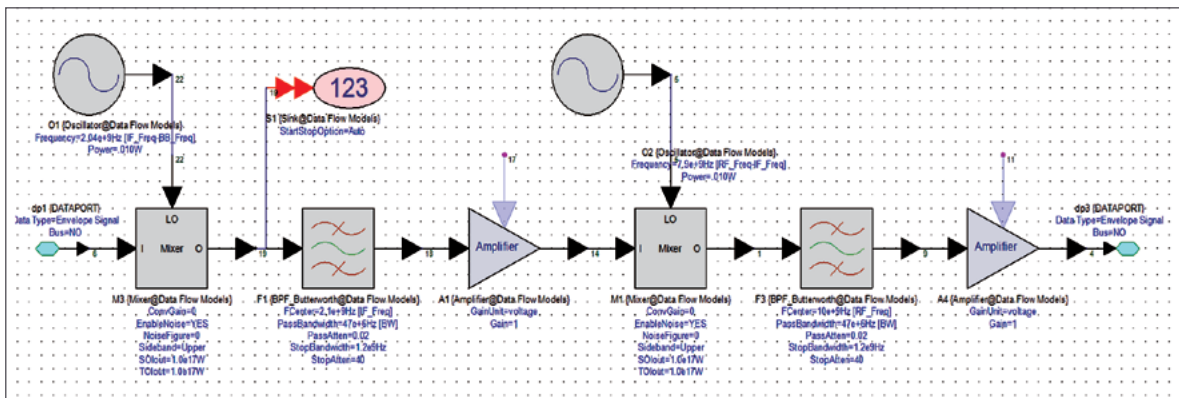
Figure 4.8. RF transmitter
