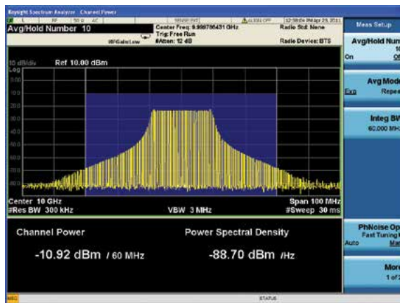
Chirped radar
