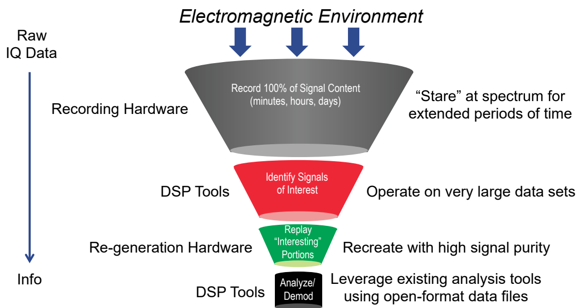
Figure 22.4. RF energy is first stored as IQ samples where DSP tools are used to identify and demodulate signals of interest. These stored IQ samples can also be used for signal playback or combined with other signal files for scenario simulation.
