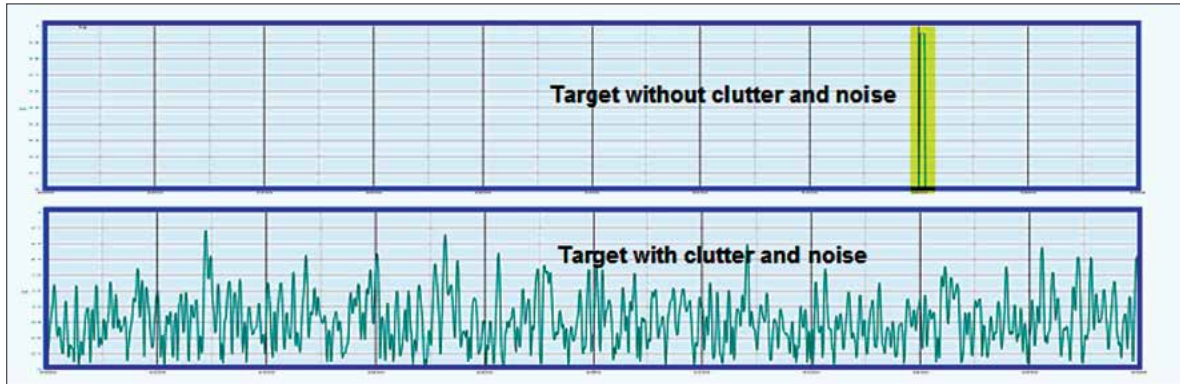
Figure 4.5. Target signal hidden by heavily cluttered environment
