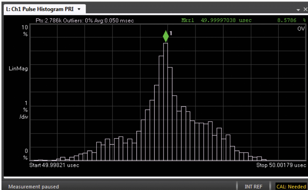
Figure 17.17. Pulse histogram
