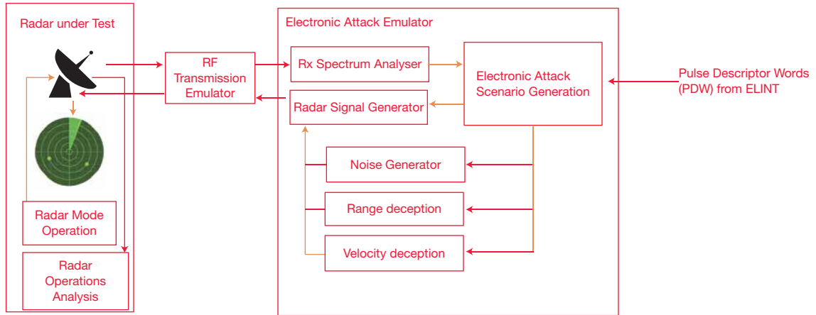
Figure 23.2. Radar test environment under jamming attack
