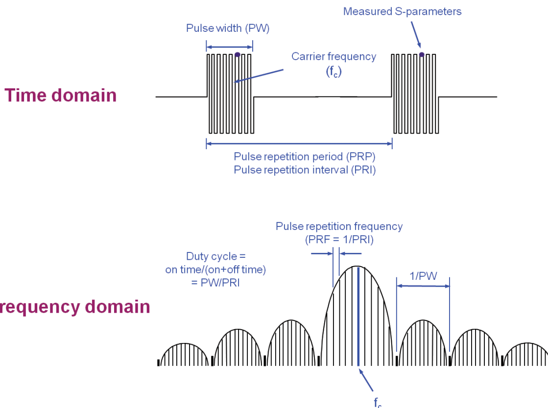
Figure 12.8. Pulsed-RF network analysis terminologies
