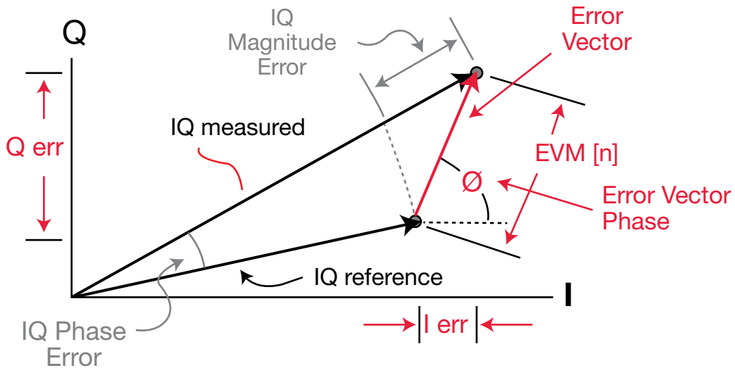
Figure 20.6. Error vector magnitude (EVM)
