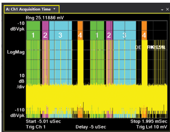
Figure 17.13. Trace types, statistics and measurements
