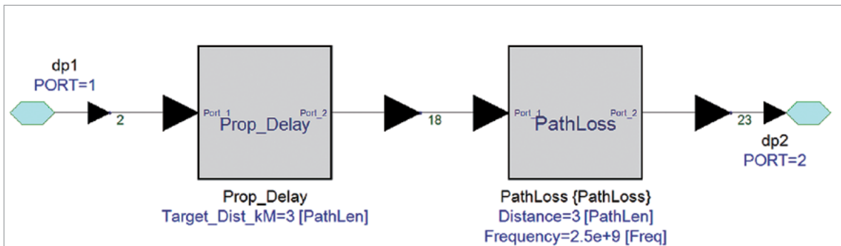
Figure 3.7b. Implementing radar propagation loss and propagation delay models
