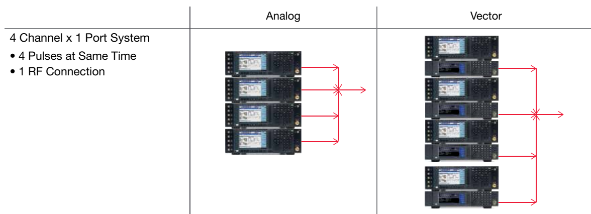
Figure 16.18. 4-channel, 1-port configurations
