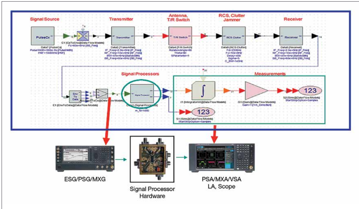
Figure 4.2. SystemVue as a platform for test
