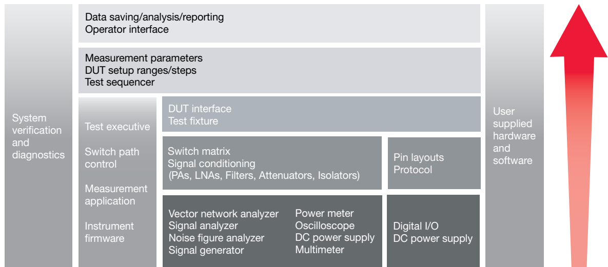
Figure 18.5. Conceptual building block for test system
