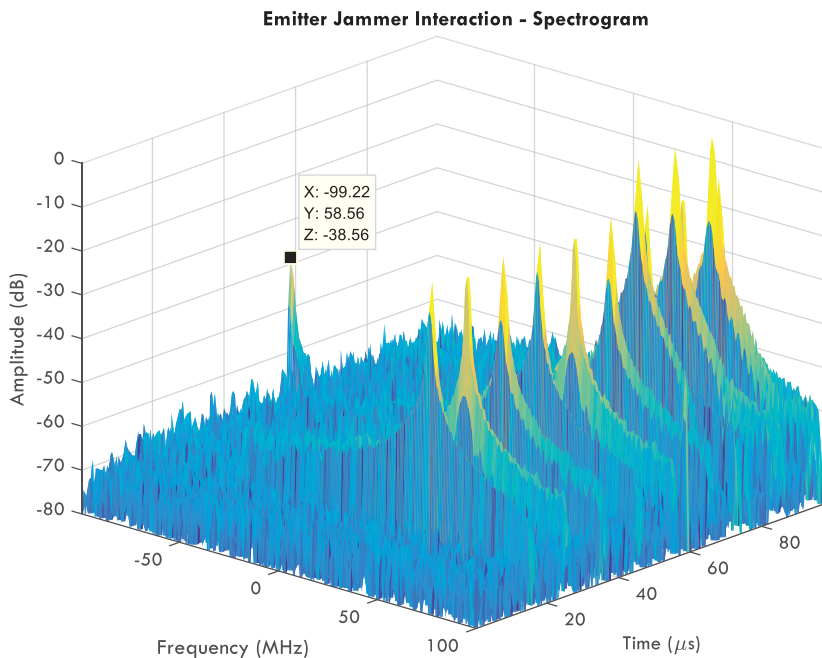
Figure 22.13. Spectrogram plot of emitter-jammer interaction.
