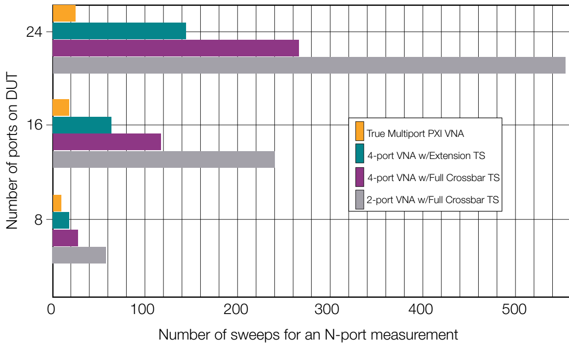
Figure 12.14. Sweeps required for multiport devices
