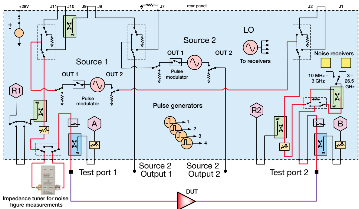
Figure 18.6. VNA architecture
