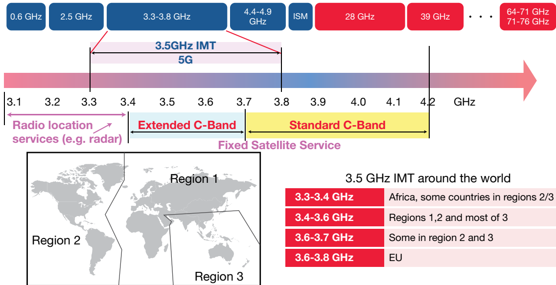
Figure 20.5. Detailed frequency range for 5G NR
