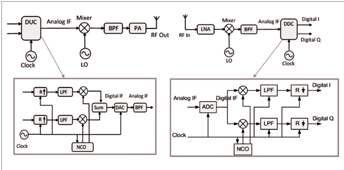
Figure 4.10. Digital up/down converters
