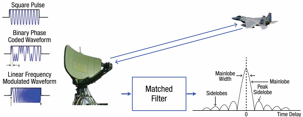
Figure 17.23. Pulse compression
