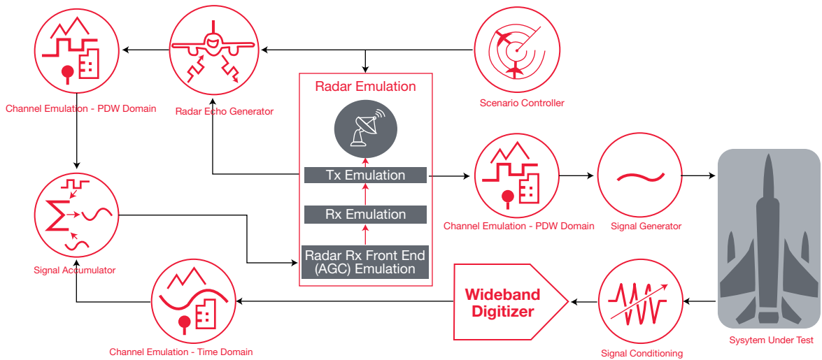
Figure 23.3. EA test environment against enemy radar
