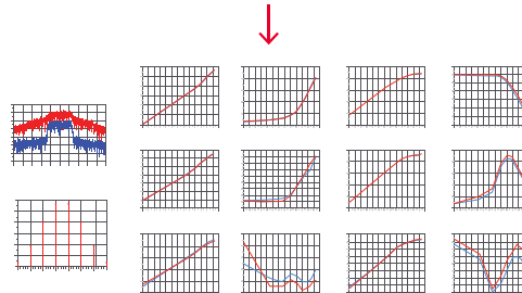
Figure 14.1. Measure complete linear and nonlinear component behavior with the Keysight NVNA, and then accurately perform simulations and optimizations with Keysight's Advanced Design System.
