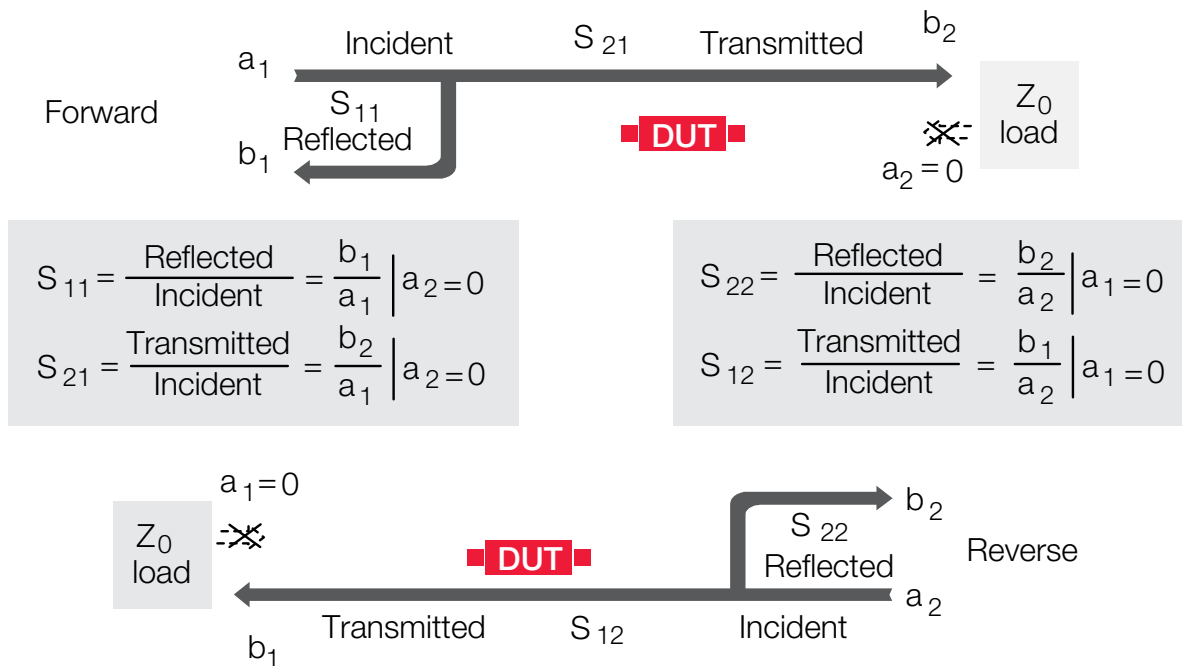
Figure 12.3. Measuring S-parameters
