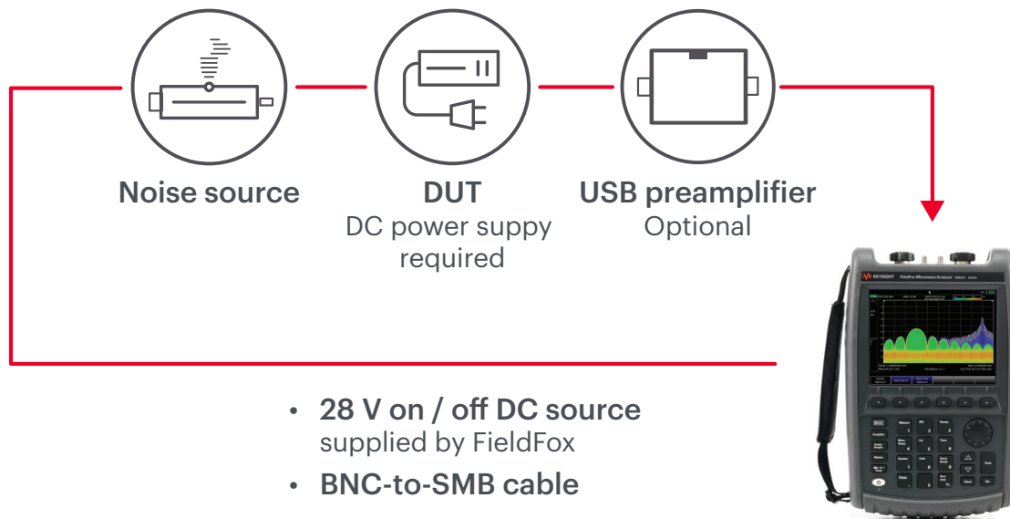
Figure 4. Noise measurement with the FieldFox handheld analyzer.
