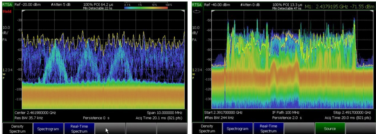
Figure 1. A Wi-Fi signal captured by a FieldFox handheld analyzer with 10 MHz bandwidth on the left and 100 MHz bandwidth on the right. With 100 MHz bandwidth, you can visualize the whole band in one display.
