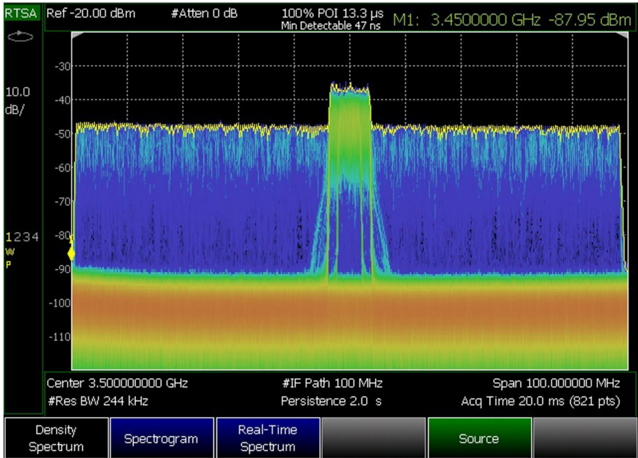
Figure 3. FieldFox's 100 MHz real-time bandwidth identifies a 5G NR signal.
