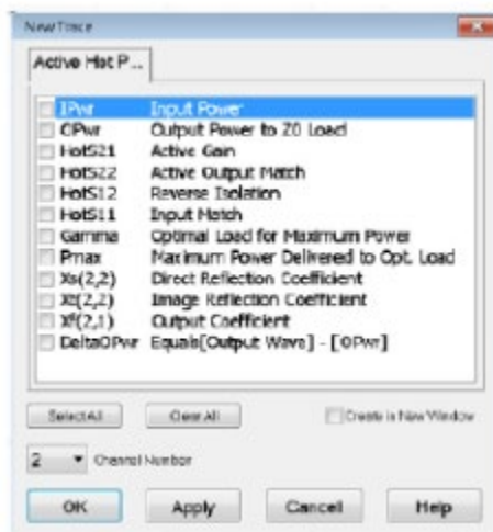
Hot S22 measurement with active parameter measurement function
