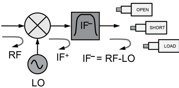
Calibration mixer/filter pair
