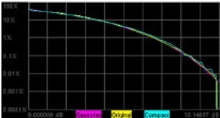
Figure 16. CCDF Comparison of the original 5G NR 100 MHz signal vs. compact test signal consisting of 10,001 tones. Share the same Power Spectral Density (PSD) and Complementary Cumulative Density Function (CCDF).
