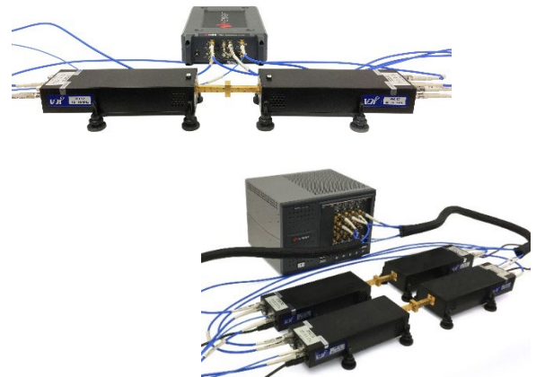
Banded VNA with Streamline Series VNA / PXI-VNAs
