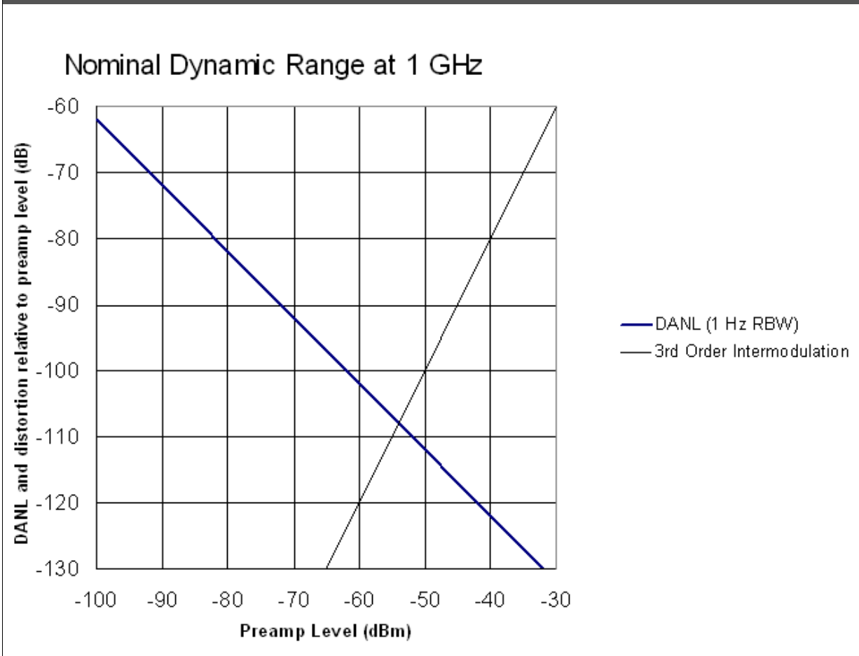
Nominal Dynamic Range at 1 GHz, Preamp On, Freq Option ≤ 526 [Plot]
